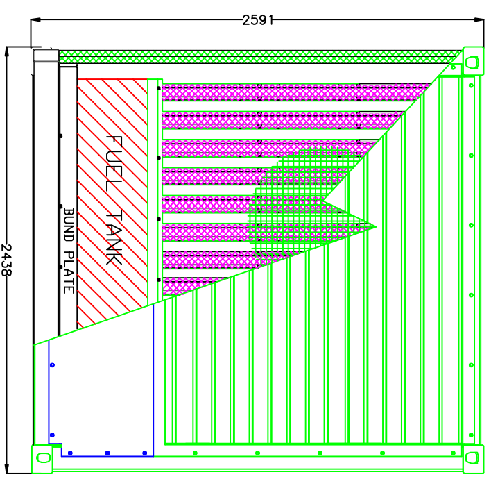
ALTERNATOR END VIEW
