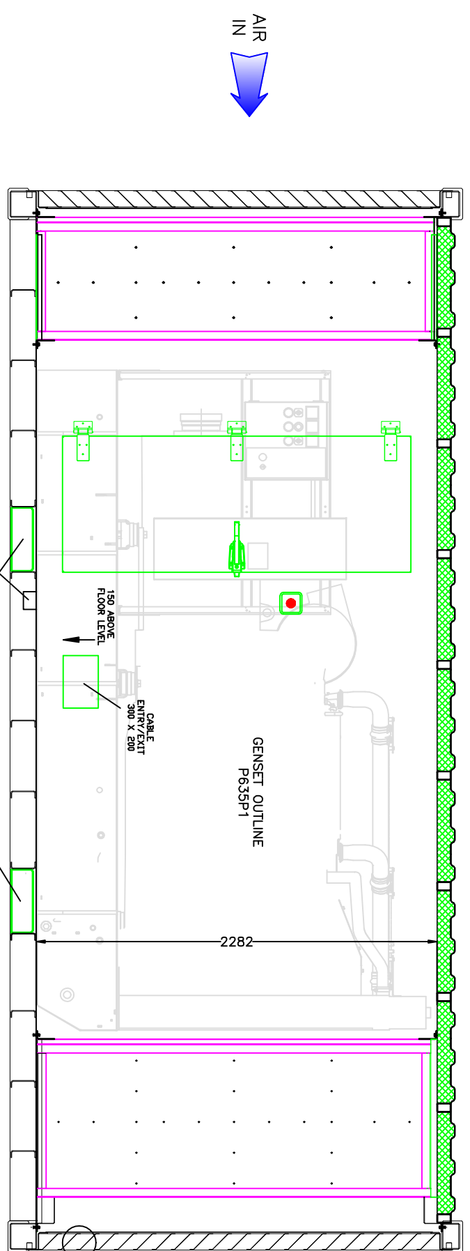
SIDE VIEW (WALL DETAIL REMOVED)
